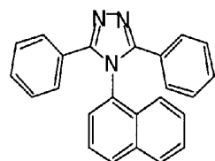
3-phenyl-4-(1-naphthyl)-5-phenyl-1,2,4-triazole
