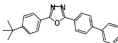
2-(4-tert-butylphenyl)-5-(4-biphenyl)-1,3,4-oxadiazole
